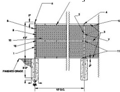
FENCE DETAIL
