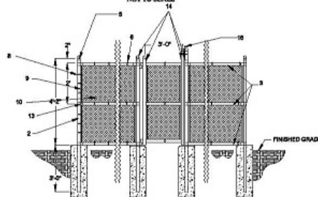
SINGLE LEAF GATE DETAIL
