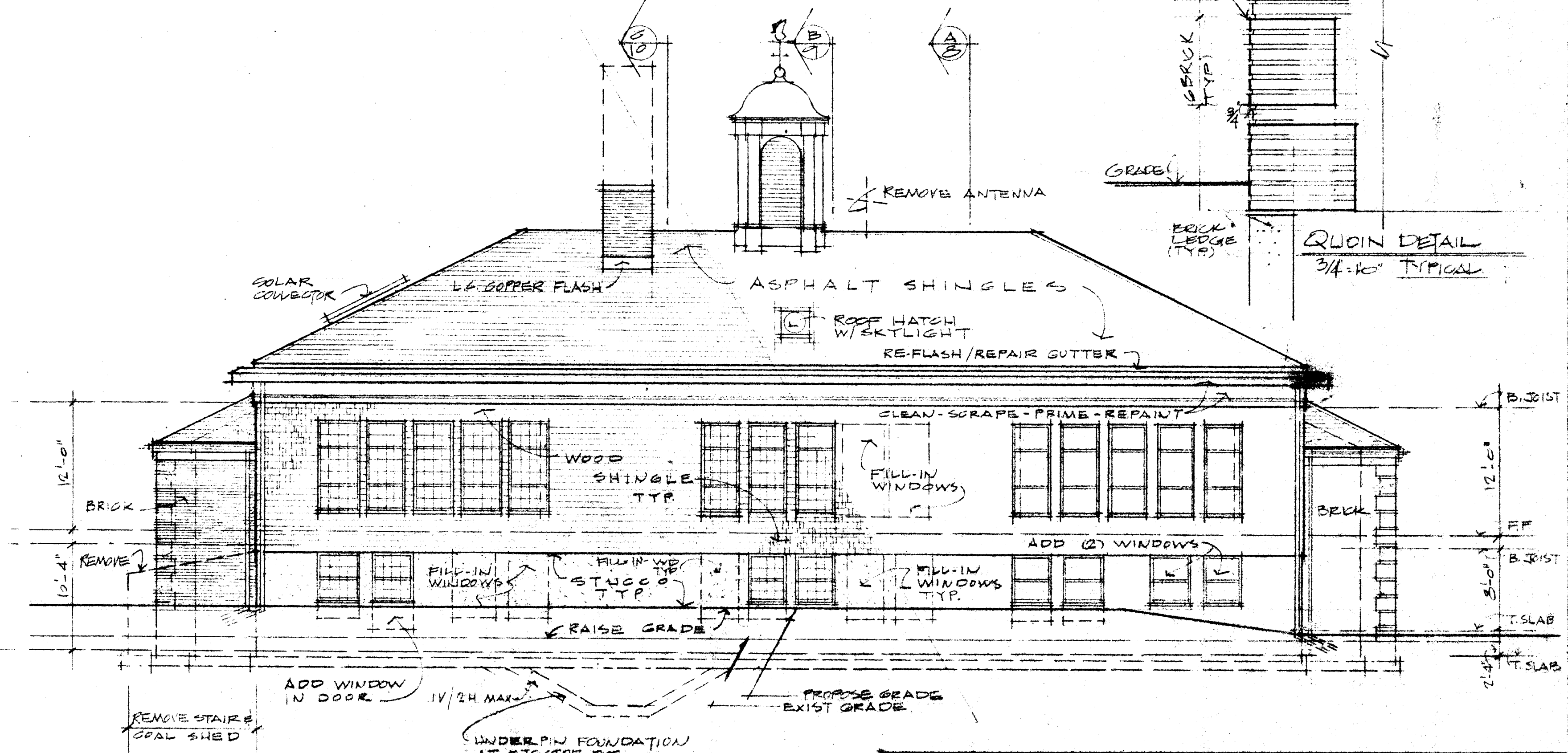
WEST ELEVATION \frac{1}{8}'' = 1'-0''
