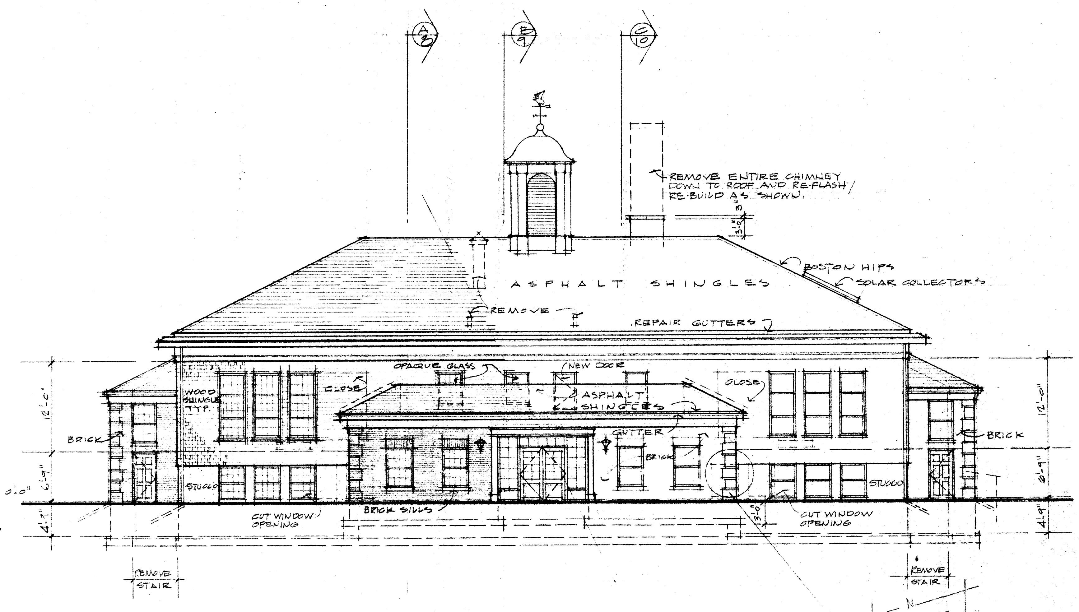
WEST ELEVATION \frac{1}{8}'' = 1'-0''
